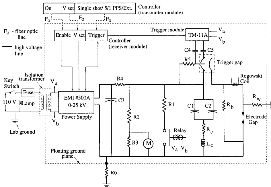
FIG. 1. High-voltage supply and control circuit. Heavy lines designate high-voltage conductors, and light lines are either control lines or are at building supply voltage (110 V).
