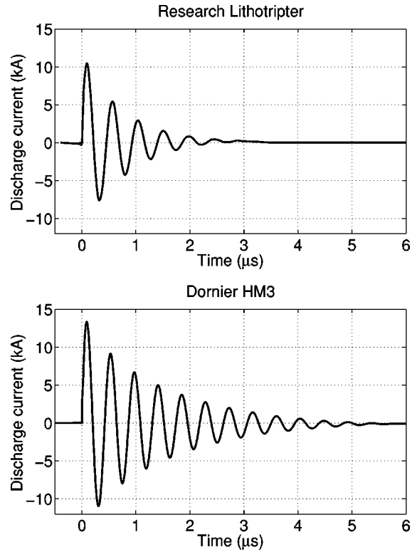
FIG. 6. Discharge current measured by the Rogowski coil. V_0=18 kV, shorted electrode. Top, GALCIT EHL; bottom, HM3-A.
