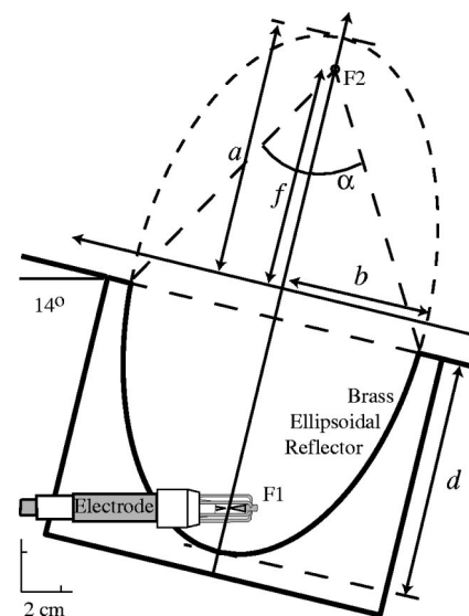
FIG. 3. Ellipsoidal reflector geometry: a = 139 mm, b = 78 mm, d = 124 mm and f = 114 mm.
