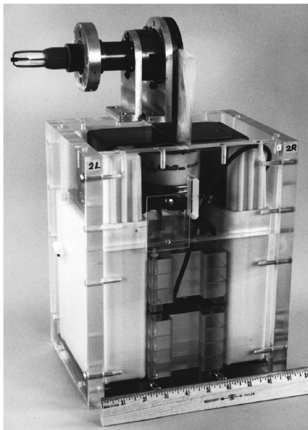
FIG. 2. Power pack assembly: (a) schematic (not to scale) and (b) photograph of a fully assembled power pack (scale is in inches; 1 in.=25.4 mm).
