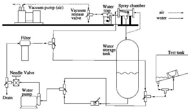
FIG. 4. Water degassing and storage system.
