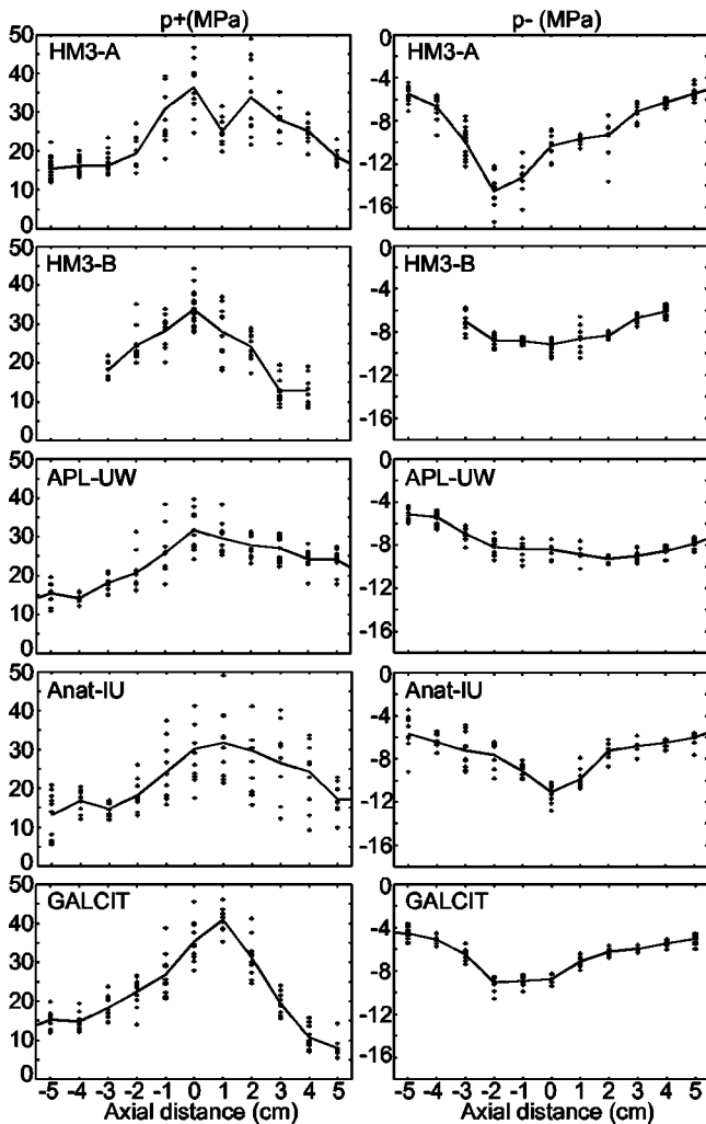
FIG. 10. Variation in p+ (left column) and p- (right column) with axial location.
