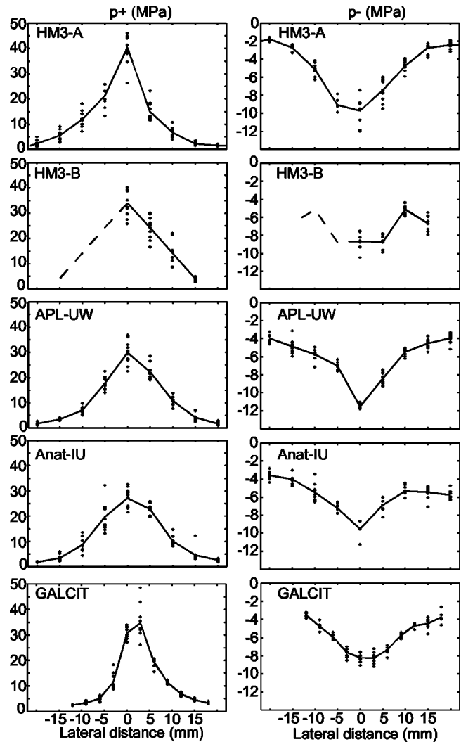
FIG. 11. Variation in p+ (left column) and p- (right column) with lateral location.
