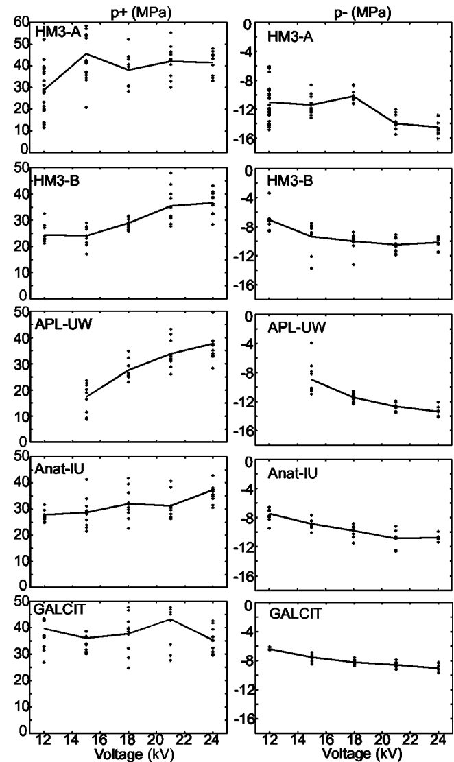
FIG. 9. Variation in p_+ (left column) and p_- (right column) with charging voltage for the five lithotripters.
