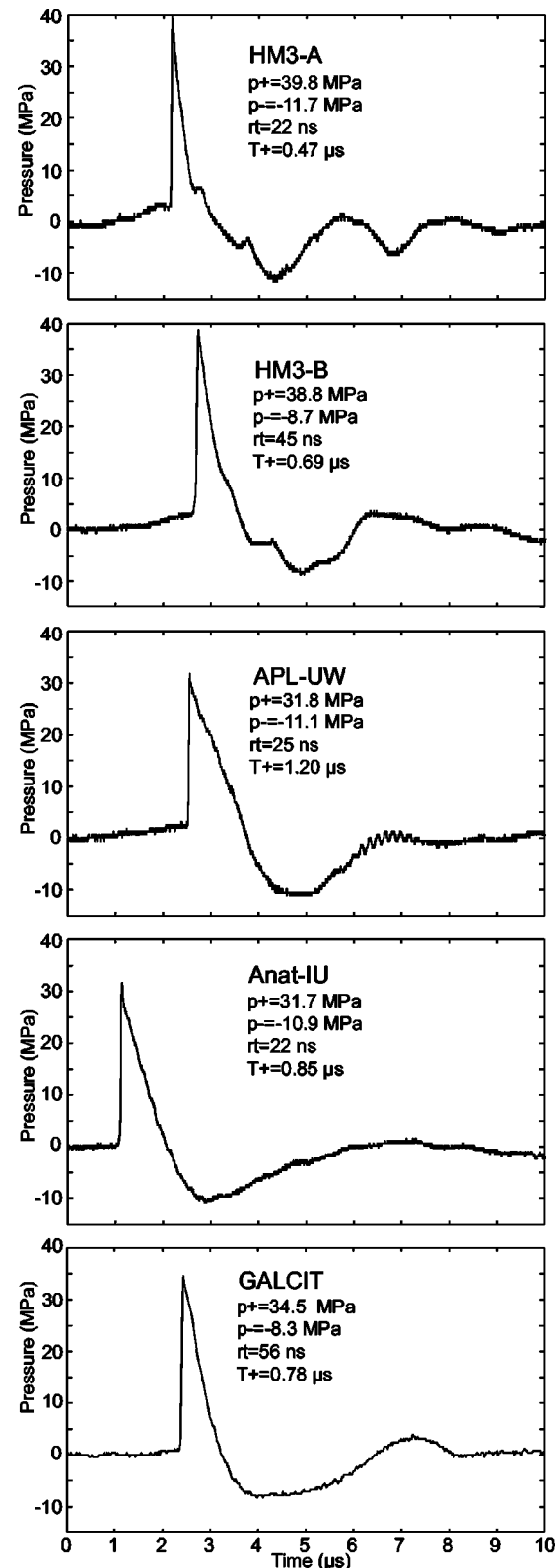
FIG. 8. Representative waveforms measured in the different lithotrippers at the geometrical focus with a discharge voltage of 18 kV.
