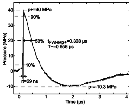
FIG. 5. Shock wave parameters: peak positive pressure p+ , peak negative pressure p- , duration of the positive phase T+ , and rise time rt .
